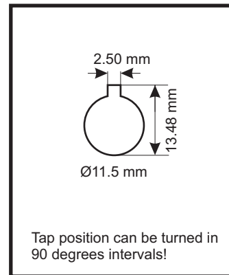
Hole Guide for Single Terminal
